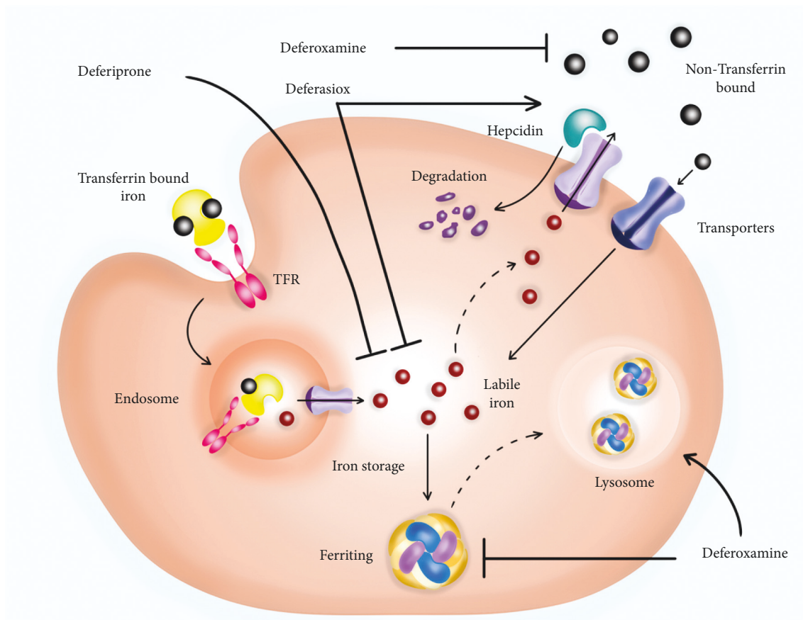
FIGURE 1: Deferoxamine, deferiprone, and deferasirox mechanism of action in the management of iron overload. Deferoxamine binds to nontransferrin bound iron or to iron found in ferritin forming a molecule which is later excreted via the kidneys. Deferoxamine also promotes ferritin degradation in lysosomes. Deferiprone and deferasirox chelate cytosolic labile iron. Besides, deferasirox can increase the levels of hepcidin that results in the degradation of ferroportin. TFR, transferrin receptor.
