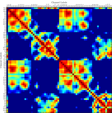
Original Correlation Matrix
