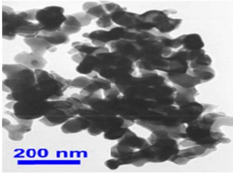
Fig. 4. TEM photograph of Al 2 O 3 particles.
