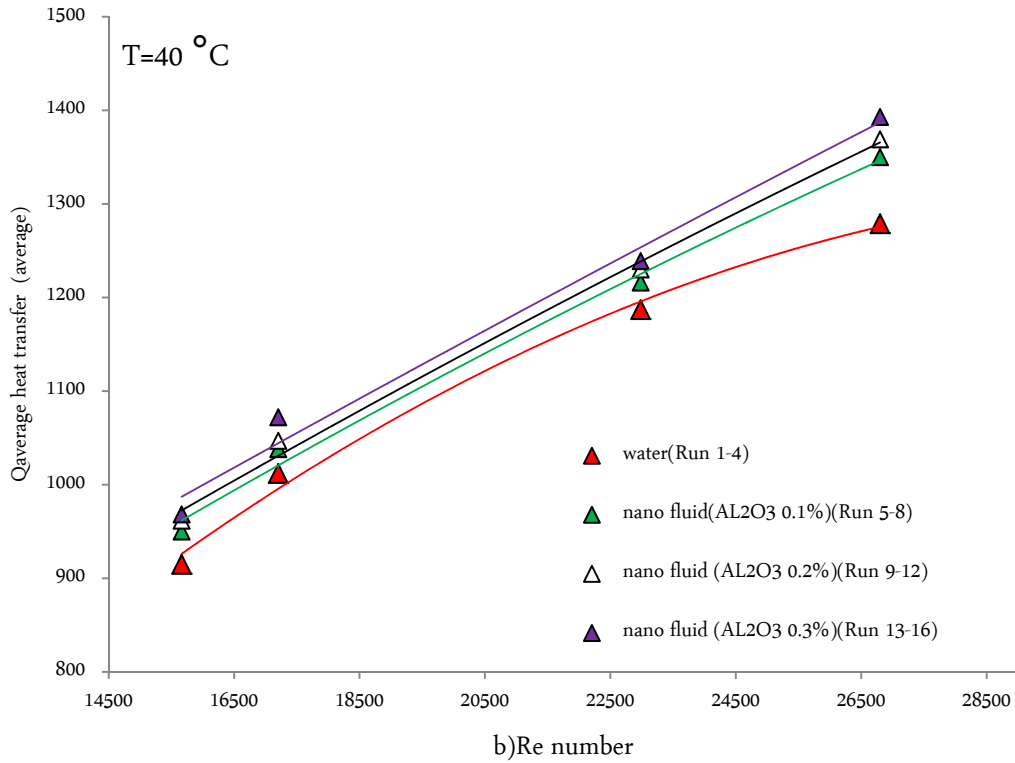
Fig.5. Average heat flow rate of the Reynolds number at a) 35 and b) 40 °C.
