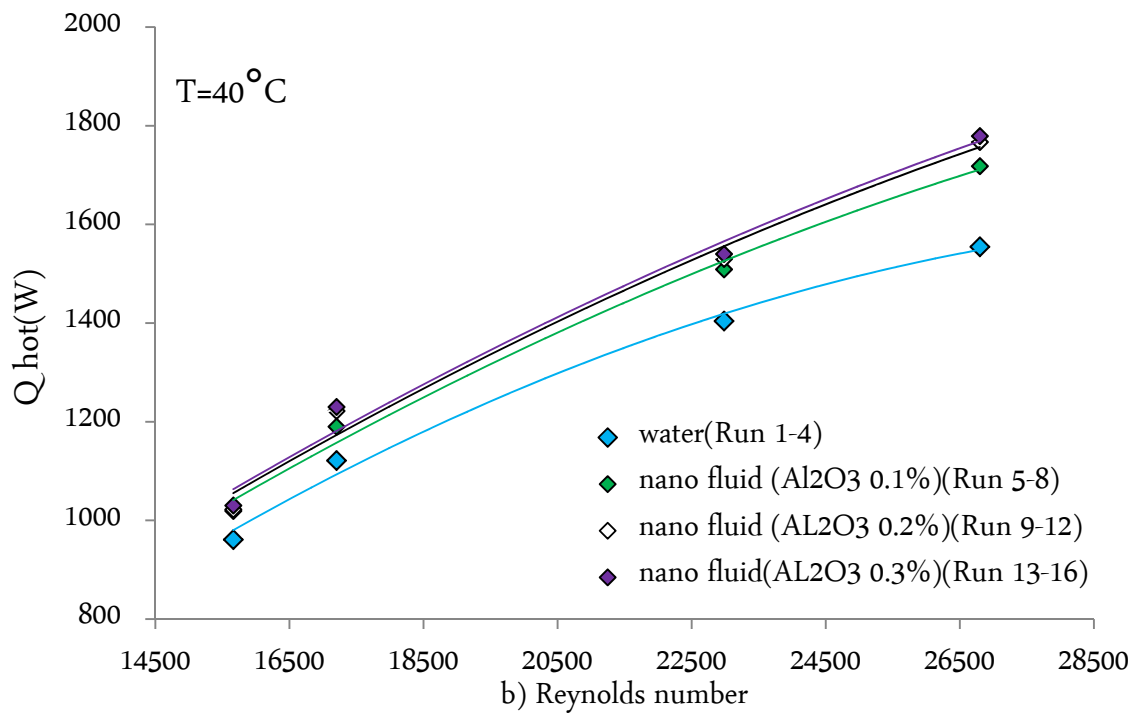
Fig.6. the rate of heat flows Reynolds numbers at a) 35 and b) 40 °C.
