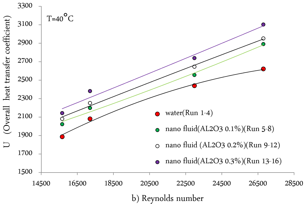
Fig.7. overall heat transfer coefficient versus Reynolds number changes at a) 35 and b) 40 °C
